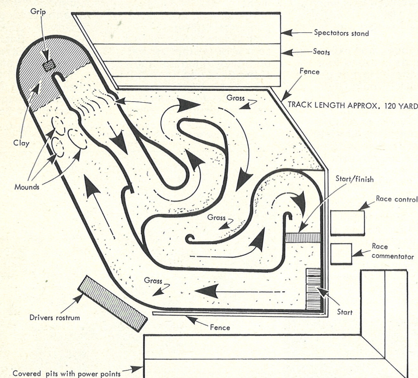
Fig. 1 Track diagram
