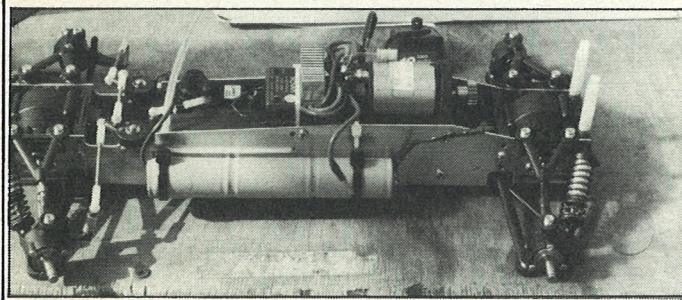
The SG/TAG 'Coyote' employs shaft drive between front and rear from an in-line motor. Ni-Cads are carried in two, three cell, sticks mounted either side of the chassis. Limited slip differentials feature front and rear.
