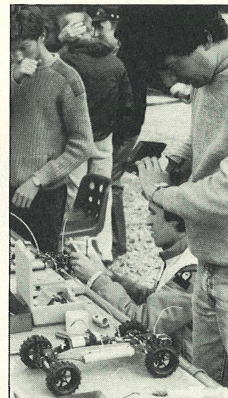
The SG/TAG 'Coyote' employs shaft drive between front and rear from an in-line motor. Ni-Cads are carried in two, three cell, sticks mounted either side of the chassis. Limited slip differentials feature front and rear.
