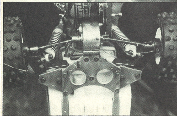
Above left: belt drive for the Benson's 'Scorpion' provided the answer to noisy and inefficient gear mesh. Left: John also produced their own rear trailing arms from steel to alloy breakages in this area. Above: Associated 'RC10' shocks provided the damping and a lexan radio crate kept the weight down. Front anti-roll bar was also fitted.
